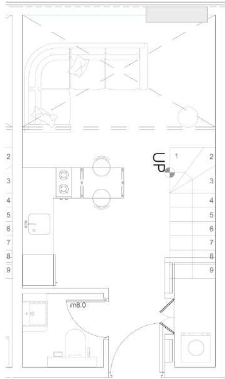
DUPLEX LOWER LEVEL
